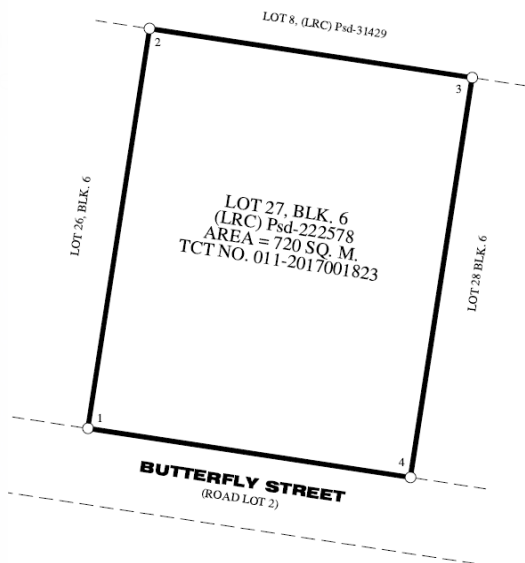
LOT AND FLAT PLANS
